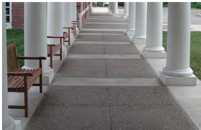
Exposed aggregate concrete paving
