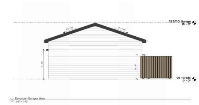
Side (Right) Elevation.
