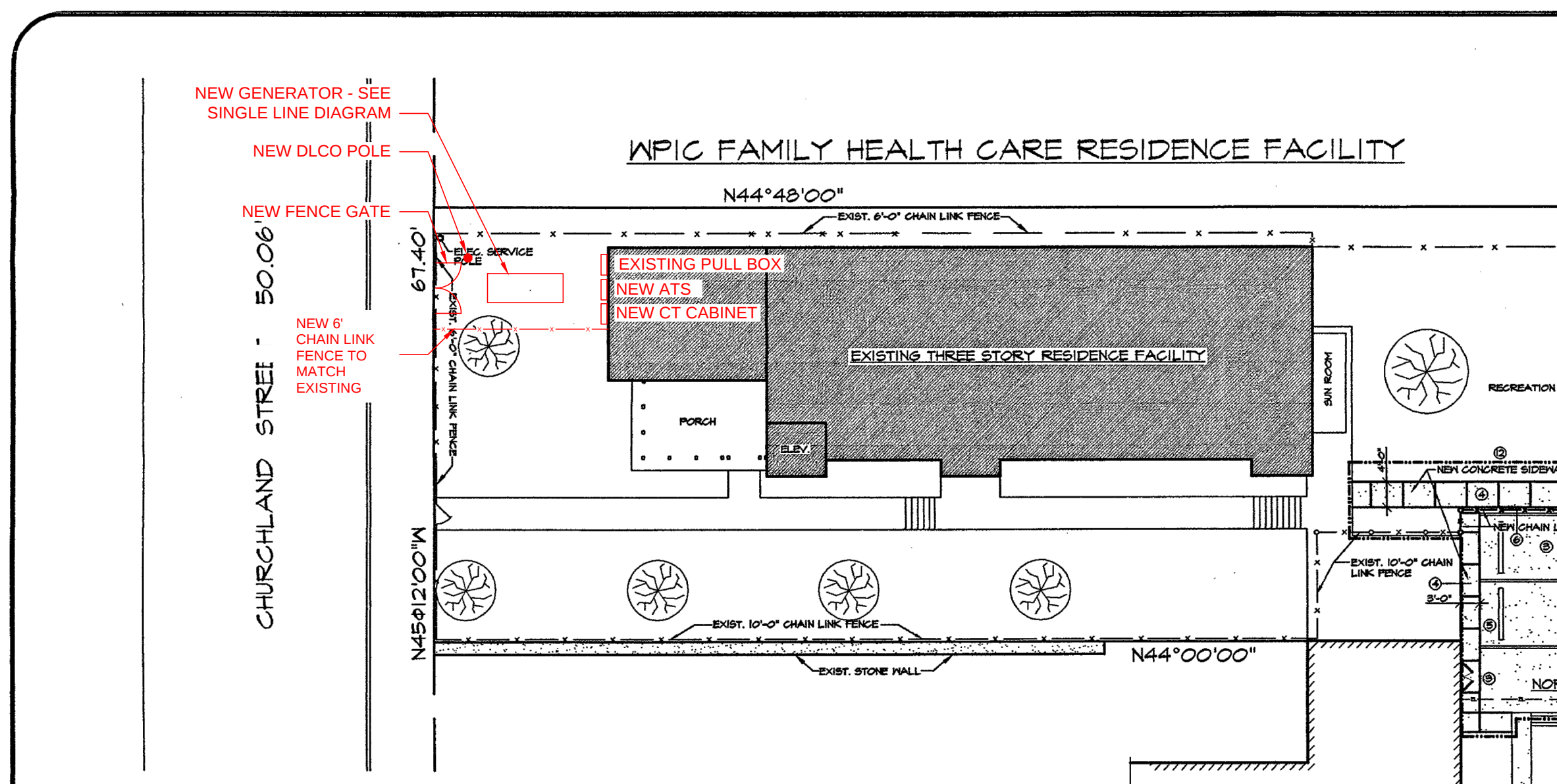
1 SITE POWER PLAN E1 SCALE: 1" = 20'
